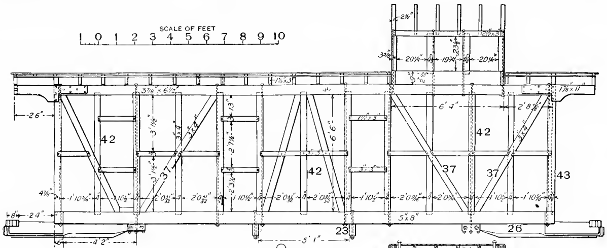
Fig. 380. Side Elevation of Frame.
